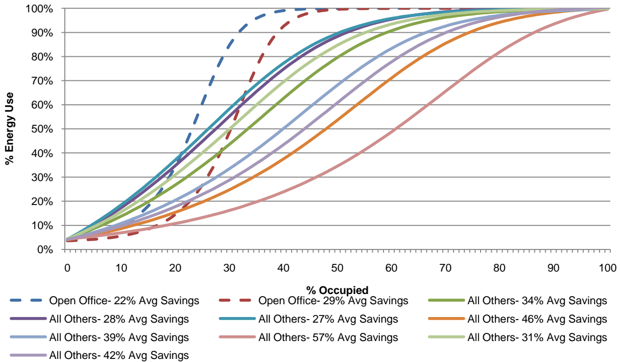
Figure 4 – Anticipated Energy Use as a Function of Occupancy and Type of Occupancy/Vacancy Sensor
