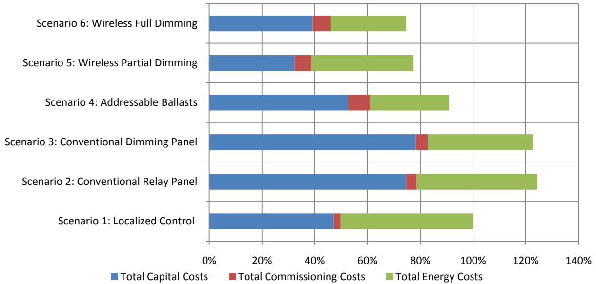
Figure 9 - Boston: Life Cycle Cost Relative to Scenario 1
