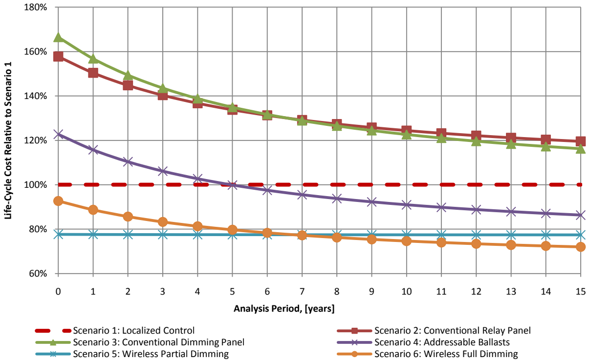
Figure 14 - Boston: Life-Cycle Cost as a Function of Analysis Period Length, Relative to Control Scenario 1
