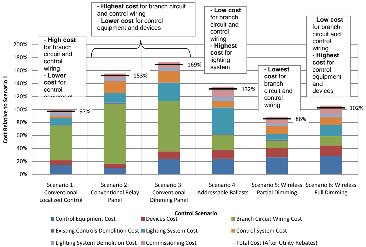
Figure 10 - Capital Cost Breakdown for Los Angeles
