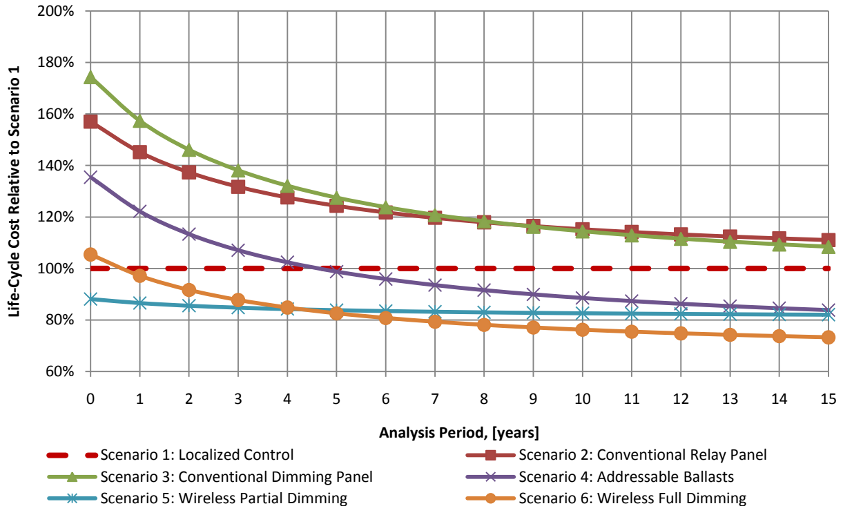
Figure 13 - Los Angeles: Life-Cycle Cost as a Function of Analysis Period Length, Relative to Control Scenario 1
