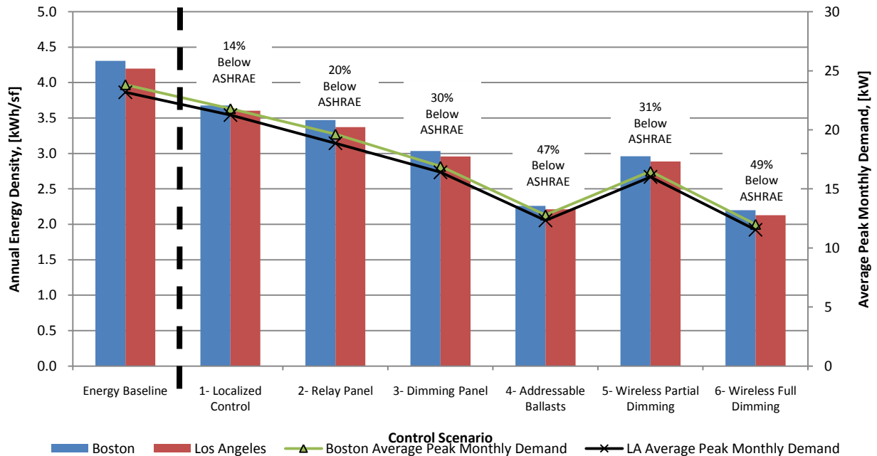
Figure 5 –Annual Energy Density and Associated Peak Monthly Demand
