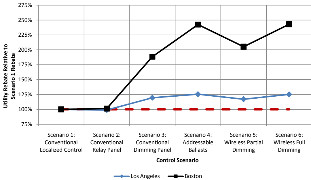
Figure 12 – Utility Rebates Relative to Control Scenario 1
