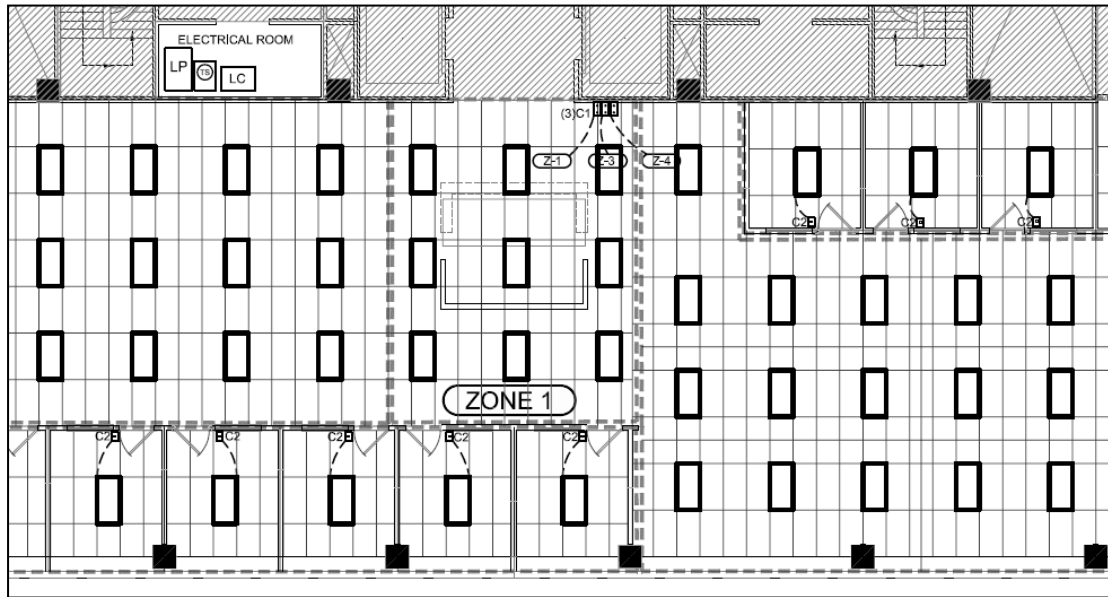
Figure 2 - Typical Luminaire Configuration
