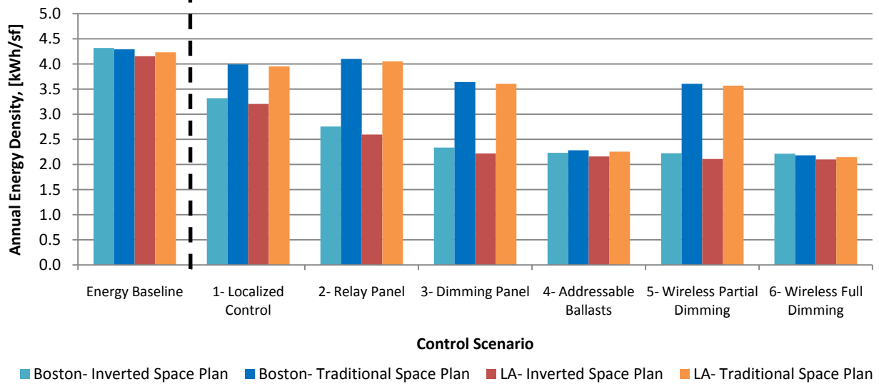
Figure 6 – Annual Energy Density, Split by Location and Space Planning
