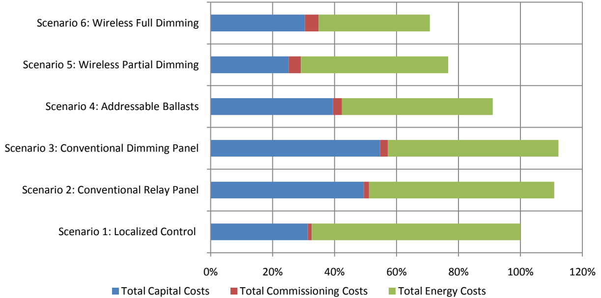
Figure 8 - Los Angeles: Life Cycle Cost Relative to Scenario 1
